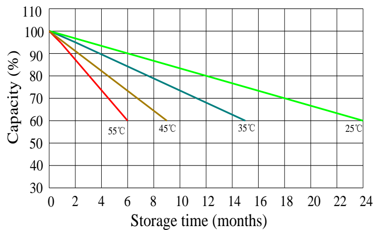
Self-discharge at different temperature
